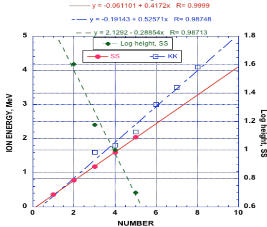
FIGURE 2. A comparison between the measurements of Karabut et al. (KK)[67] and Storms and Scanlan (SS)[68] showing the kinetic energy of the claimed ^4H^+ emissions resulting from the fusion of deuterium. The NUMBER identifies each value in a series of energy sets that are separated from each other by the
